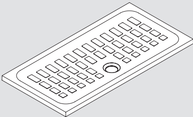
140x70xH4 cm CBPD14007040 € 500,00
