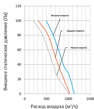
SYSPLIT DUCT 18 HP Q N
