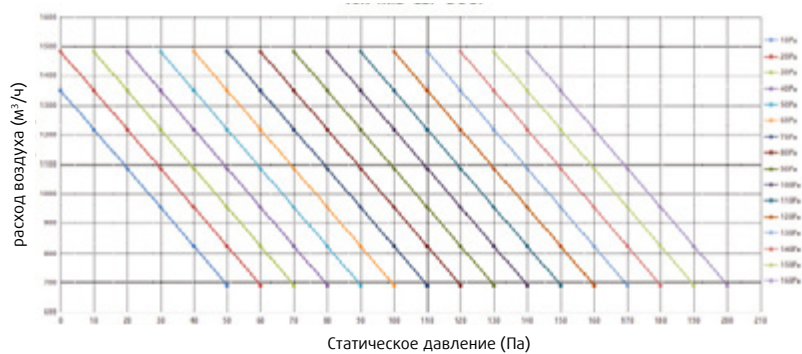
SYSPLIT DUCT EVO 18 HP Q
