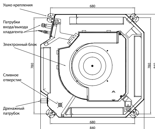
SYSPLIT CASSETTE 24-60 HP Q/R
