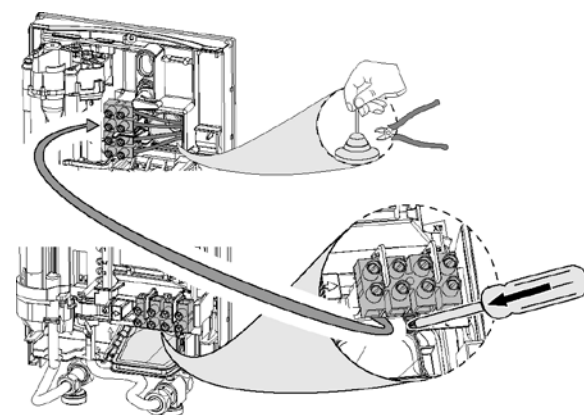
Power supply from above
