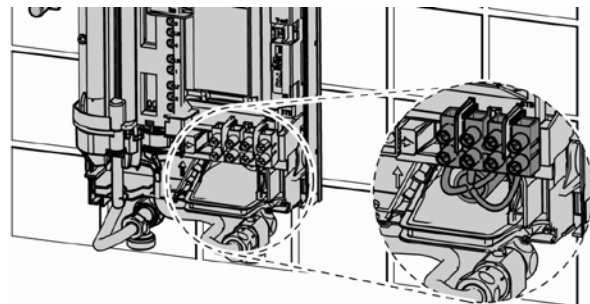
Power connection
