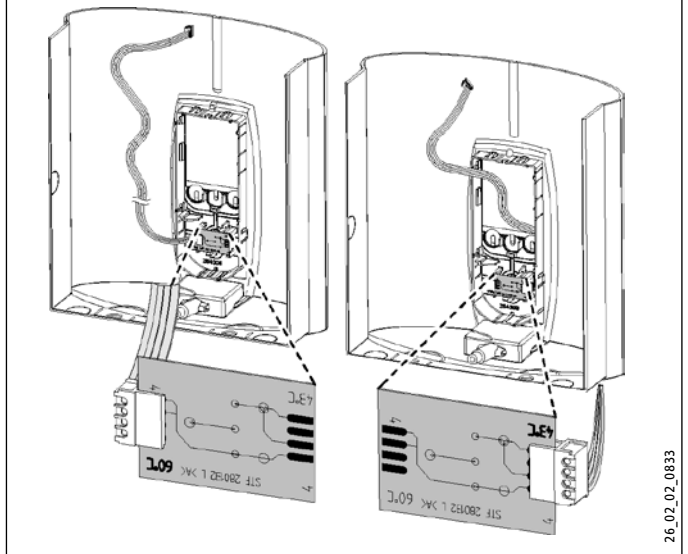
Setting the temperature limit / anti-scalding protection
