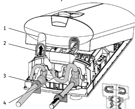
Installation information for taps for finished walls
