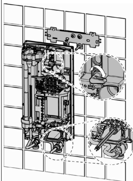
Mounting the appliance
