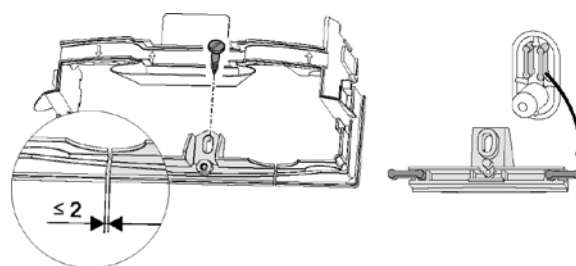
Installation with split lower part
