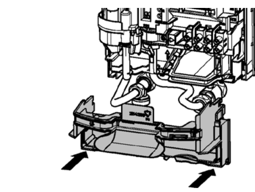
Installing and securing lower part of back panel
