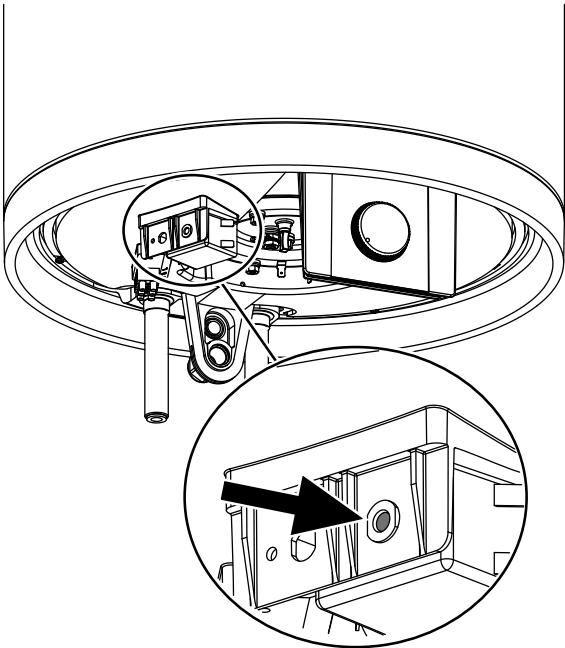
Reset key, high limit safety cut-out
