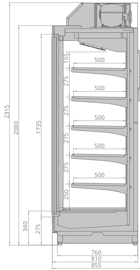
VR2080.800 ESC Plug-in
