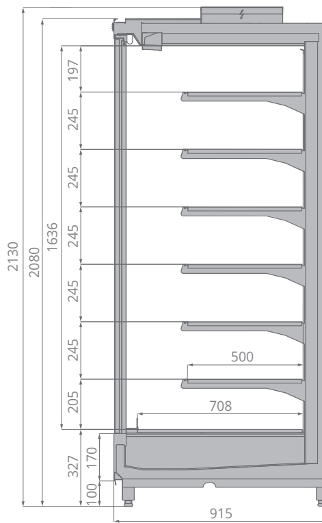
TESEY COMPACT ESC
