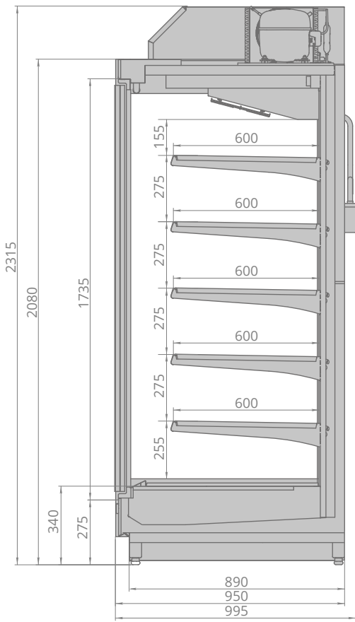
VR2080.950 ESC Plug-in
