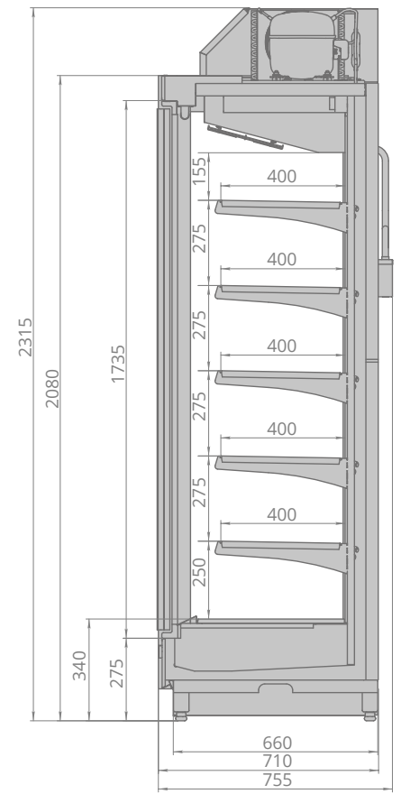
VR2080.700 ESC Plug-in
